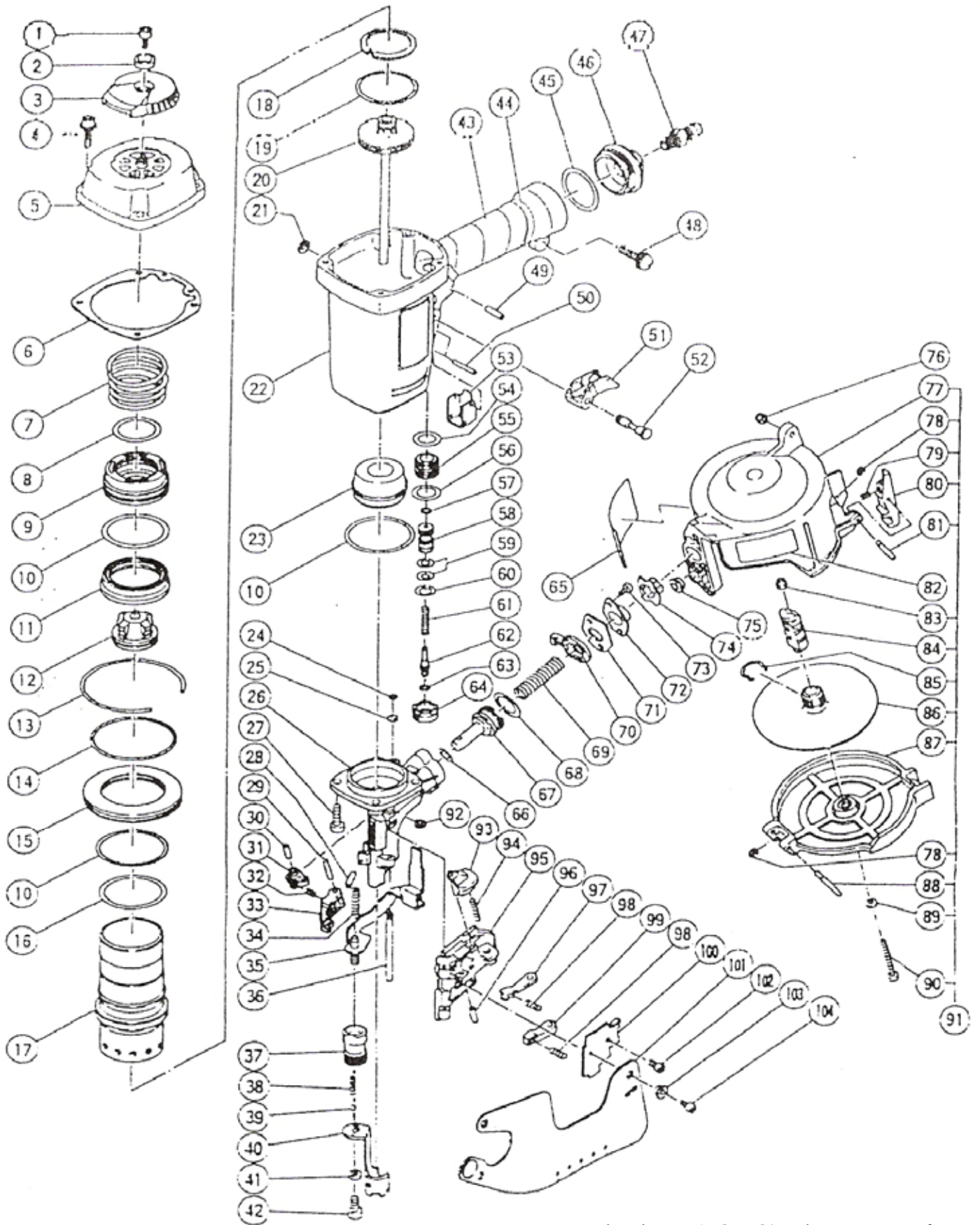
Model 610 Schematic
